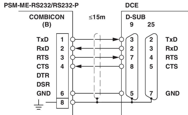
Figure 11 Connection to a DCE device
