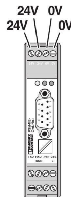
Figure 15 Connecting the supply voltage
