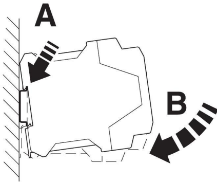
Figure 13 Mounting on a DIN rail
