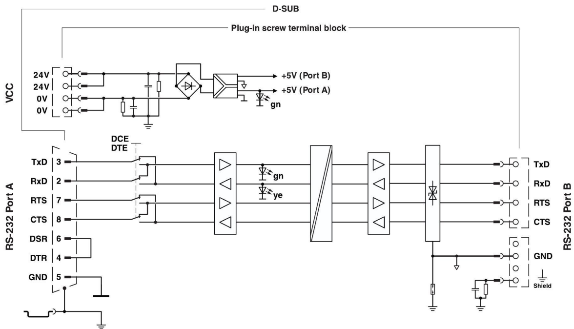
Figure 4 Block diagram
