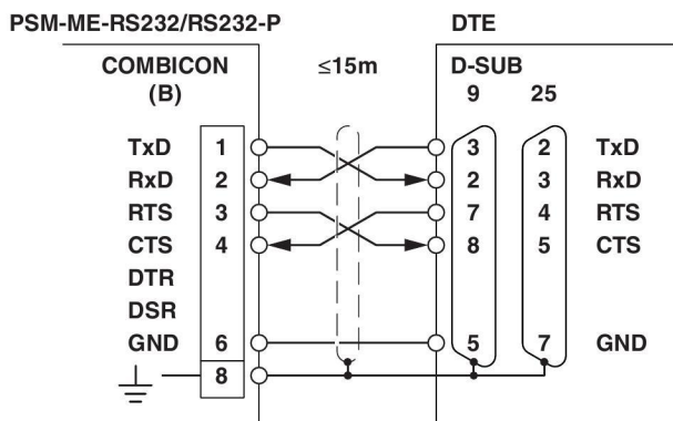
Figure 10 Connection to a DTE device
