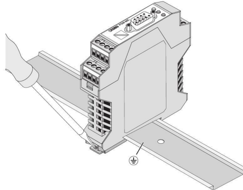
Figure 14 Removal
